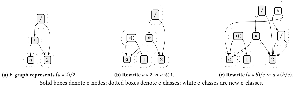
Figure 1: Applying rewrites over an example e-graph (adapted from [70])
