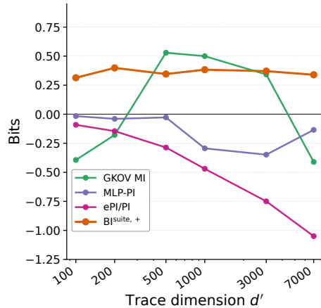
Fig. 1: The curves show metric values on CHES-CTF-2025 as the trace dimension increases from 100 to 7,000. The BI curve illustrates numerical stability when preprocessing uses the mean of the attack traces. Extending these results to a PAC guarantee requires establishing independence between preprocessing and the traces used for certification.
