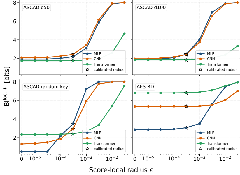
Fig. 2: The curves show local-family BI upper bounds for separate neighborhoods around twelve selected reference models. At \varepsilon_{\text{cal}} = 3 \cdot 10^{-4} , all upper bounds are below eight bits. The ASCAD upper bounds range from 1.76 to 3.48 bits. On AES-RD, the upper bounds for the neighborhoods around the MLP, CNN, and Transformer are 3.07, 5.36, and 6.83 bits, respectively.
