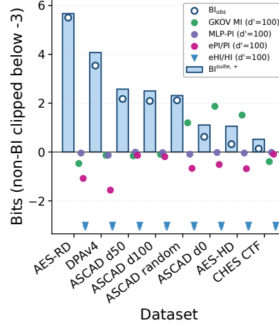
Fig. 5: The figure compares empirical BI values and finite-suite BI upper bounds with estimates computed at reduced trace dimension d' = 100 . The plotted BI values use different evaluation settings from Table 7. Values below the lower display limit are clipped, and the CHES upper bound remains a numerical diagnostic.
