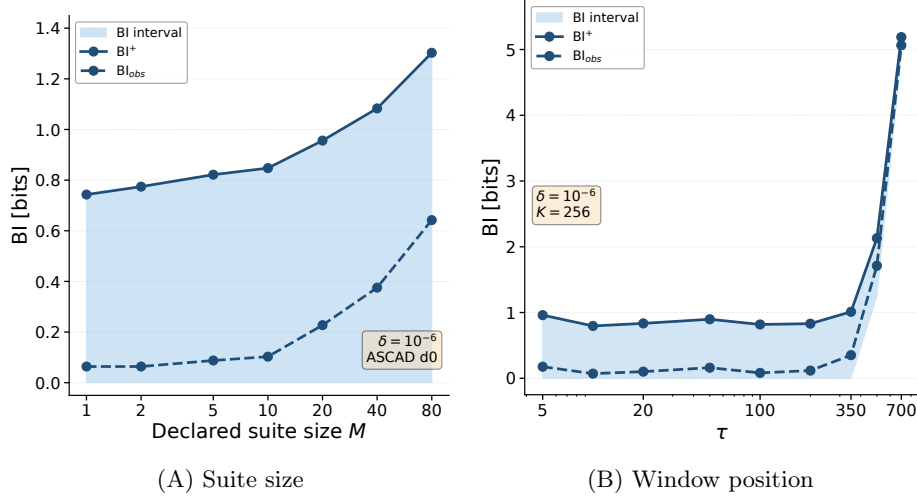
Fig. 6: (A) Empirical BI and upper bounds for the first M models in a fixed ASCAD d0 suite evaluated on 25,000 attack traces. As M increases from one to 80, empirical BI increases from 0.064 to 0.642 bits, while the upper bound increases from 0.743 to 1.303 bits. This experiment uses different evaluation settings from the main table; the reported bounds apply separately to each evaluated suite size. (B) Mean empirical BI and recomputed lower and upper bounds across five random seeds in a separate ASCAD d0 CNN experiment. Each run evaluates a window position selected using profiling traces.
