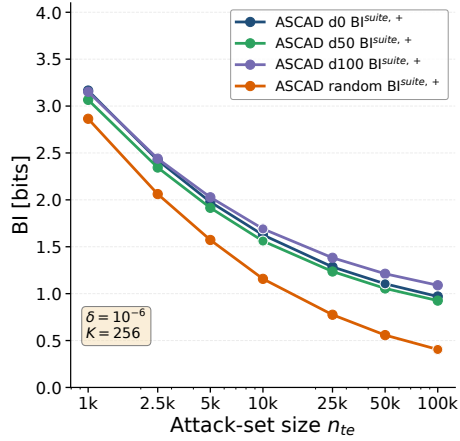
Fig. 4: The curves show BI upper bounds for four ASCAD variants as the assumed attack-set size increases at fixed empirical recovery probabilities and suite sizes.
