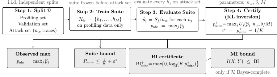
Fig. 3: The diagram illustrates finite-suite certification with failure probability \delta/M assigned to each model’s upper confidence bound. The procedure above also gives a two-sided suite interval using \delta/(2M) for each one-sided bound and a separate local-family certificate using relaxed-margin counts. Interpreting BI as an upper bound on mutual information additionally requires Bayes-completeness.
