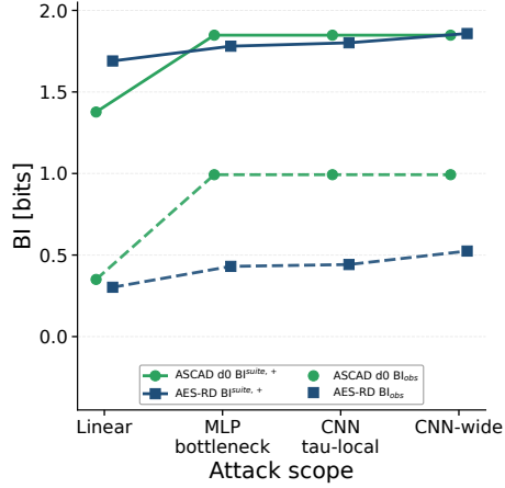
Fig. 7: The curves show empirical BI values and upper bounds as the evaluated attacker families expand to include additional architectures. A constant empirical maximum describes only the tested models and does not establish Bayes-completeness or extend the certificate to unevaluated models.
