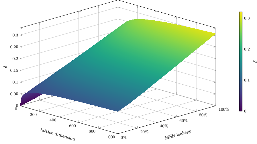
Fig. 5. Finite-dimensional bounds under MSB leakage of p + q .
