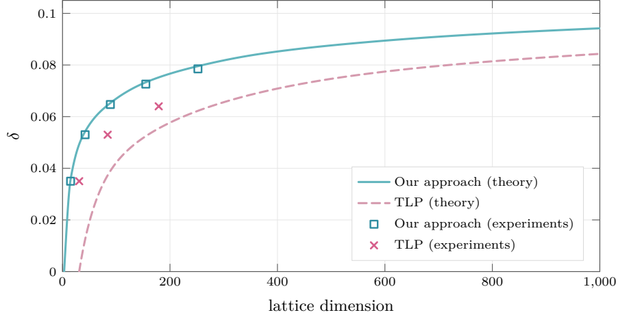
Fig. 1. Finite-dimensional bounds of our approach and the TLP attack.
