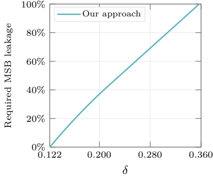
Fig. 2. Required MSB leakage of p + q .
