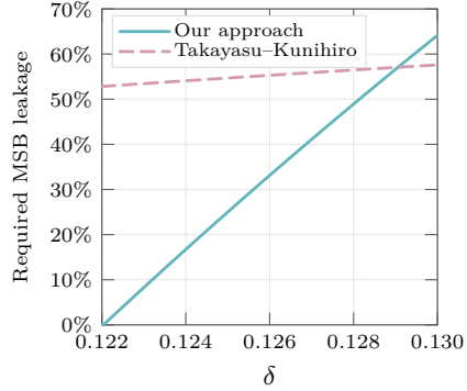
Fig. 3. Required MSB leakage of d_p, d_q .
