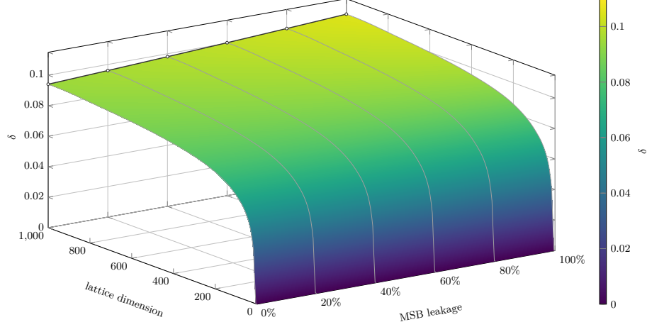
Fig. 6. Finite-dimensional bounds under MSB leakage of d_p, d_q .
