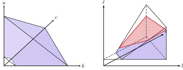
Fig. 4. Polytopes for \mathcal{M}_{\text{core}} (left) and \mathcal{M}_{\text{tail}} (right) for fixed t .
