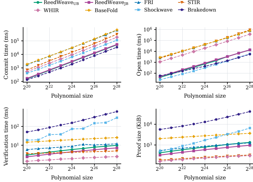
Fig. 5. Single-thread PCS performance over Goldilocks at rate 1/4 and a 100-bit security target. Brakedown retains its native rate of approximately 0.657. Points are averages of five measurements. Vertical axes are logarithmic. Lower is better.
