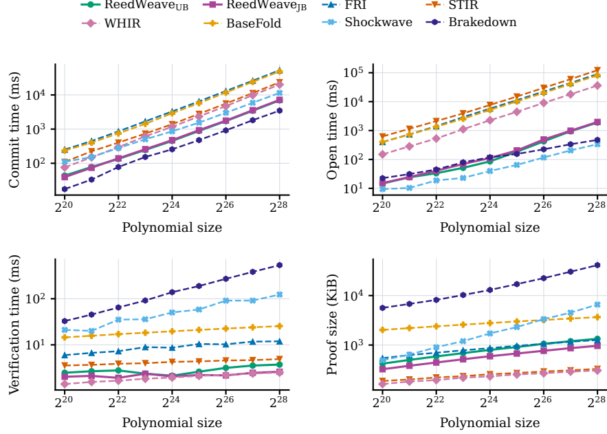
Fig. 3. PCS performance at initial code rate 1/4, with the same field, thread count, input-size convention, and averaging method as Figure 2. Brakedown retains its rate of approximately 0.657, so its curve is unchanged. Vertical axes are logarithmic. Lower is better.
