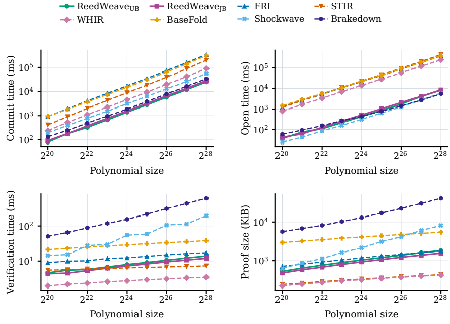
Fig. 4. Single-thread PCS performance over Goldilocks at rate 1/2 and a 100-bit security target. Brakedown uses rate approximately 0.657. Points are averages of five measurements. Vertical axes are logarithmic. Lower is better.
