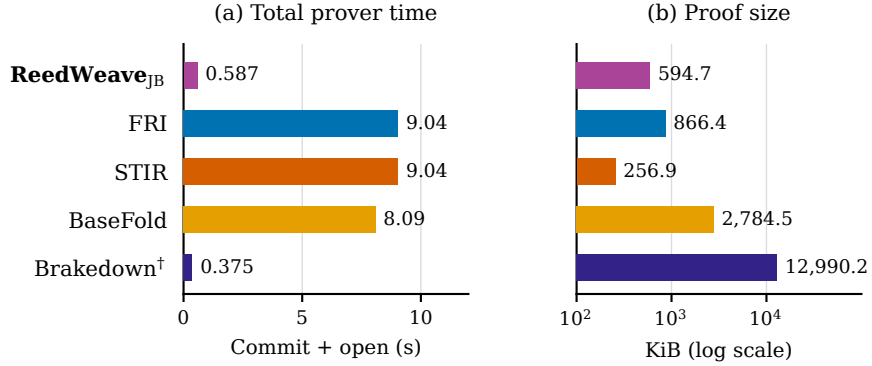
Fig. 1. PCS costs at d = 2^{24} over Goldilocks, targeting 100-bit security with 32 threads. Values are averages of five measurements. The rate is 1/4 , except for Brakedown † , which uses approximately 0.657. ReedWeave JB uses m = 64 , requiring subgroup order 2^{20} rather than 2^{26} for direct encoding. Total prover time is commitment plus opening. Proof sizes include commitments and use a logarithmic axis. Lower is better.
