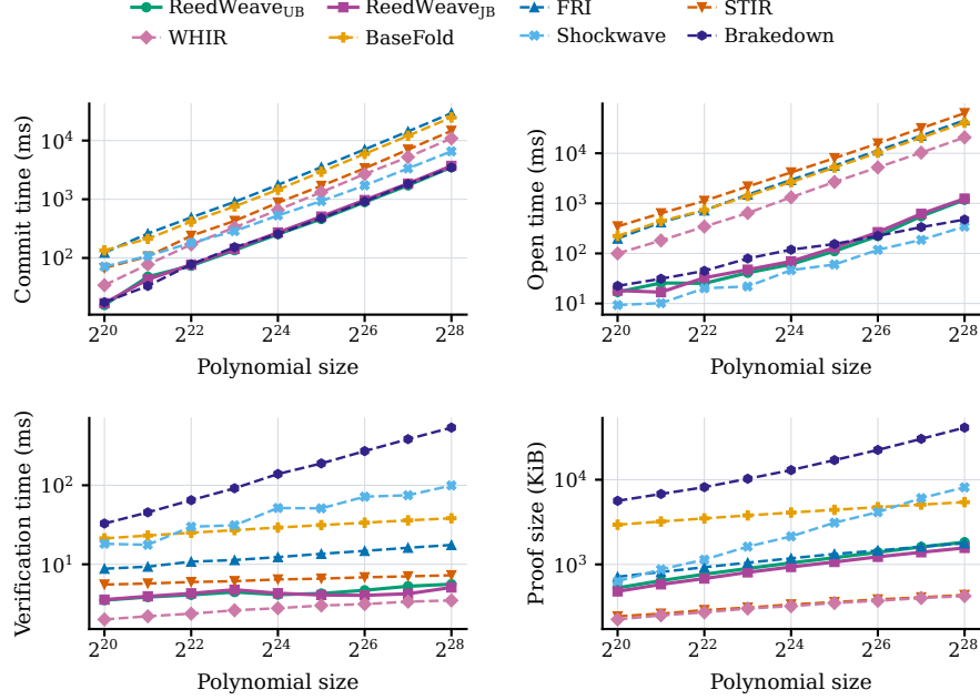
Fig. 2. PCS performance over Goldilocks at initial rate 1/2 , targeting 100-bit security with 32 threads. Points are averages of five measurements. Brakedown uses rate approximately 0.657. Vertical axes are logarithmic. Lower is better.
