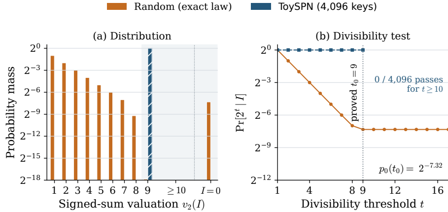
Fig. 2: Signed integral sums for the 3-round ToySPN. The bound holds for every key. The cipher distribution is empirical. Zero sums satisfy every divisibility threshold and are excluded from the pooled finite bin.
