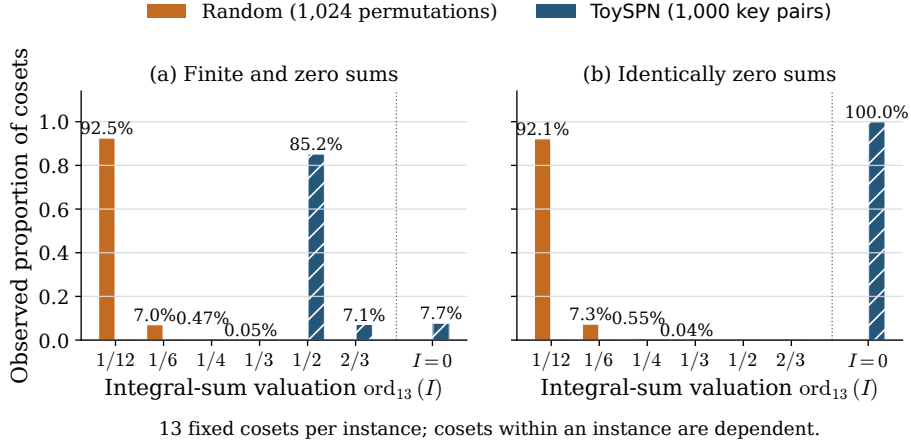
Fig. 1: Prime-field ToySPN versus random permutations. Both panels use the same independently sampled round-key pairs and random permutations. The separation in (a) is empirical. The vanishing in (b) also has a symbolic proof.
