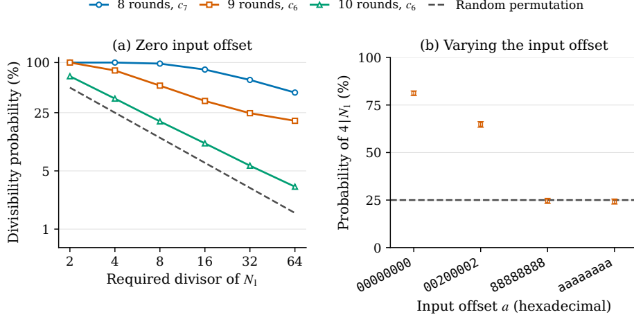
Fig. 19: Probabilistic one-count divisibility on SIMON32/64 with active mask 55555555 and data complexity 2^{16} . Panel (a): zero offset, 10,000 keys per curve, logarithmic vertical axis. Panel (b): 9 rounds, output c_6 , the same 4,000 keys at each offset. Error bars in (b) are pointwise 95% Wilson intervals, not simultaneous bands. In (a), each interval extends less than one percentage point from its estimate and is omitted for clarity. Gray dashed lines give the numerically evaluated random-permutation probabilities.
