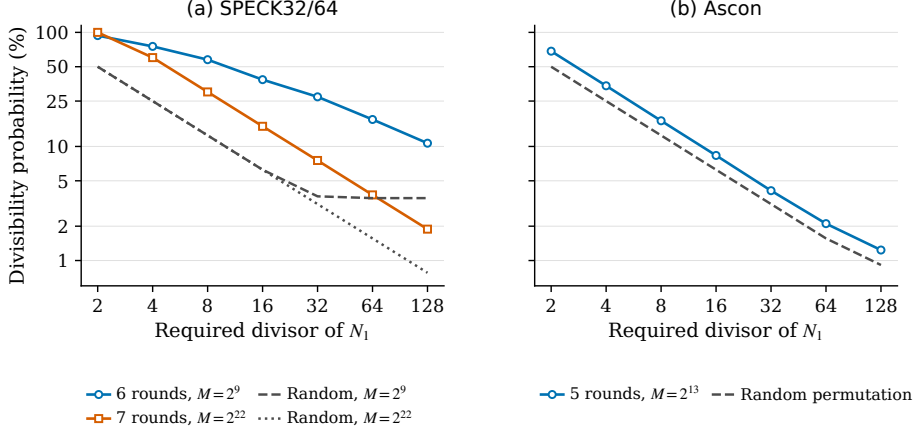
Fig. 16: SPECK32/64 and Ascon divisibility probabilities, following the conventions of Figure 14. SPECK round counts include the input-side extension.
