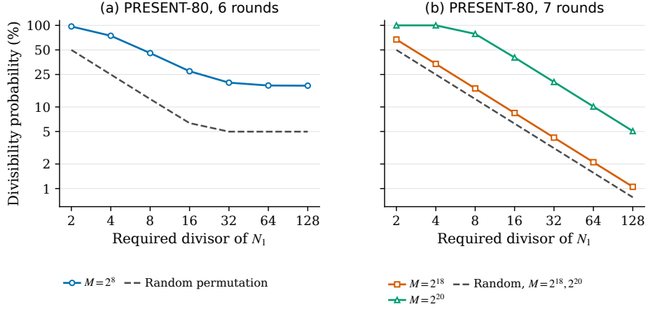
Fig. 14: PRESENT-80 divisibility probabilities at 6 and 7 rounds from Table 53, with logarithmic vertical axes. Solid marked curves show observations. Gray curves show random-permutation probabilities at the same data complexity M .
