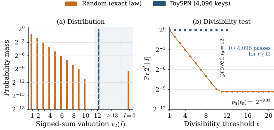
Fig. 3: 4-round, five-S-box ToySPN comparison for U = \langle 00b00 \rangle and \beta = 10000 . The data complexity is 2^{19} per coset. Each key contributes one observation because the two cosets have equal signed-sum valuations.
