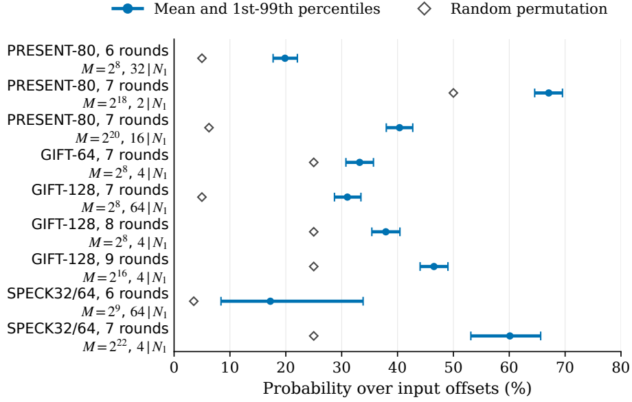
Fig. 17: Means and 1st–99th percentile ranges of per-key estimates of q_t(K) for the events in Table 52. The ranges include offset-sampling variation except for 7-round SPECK32/64. They are not confidence intervals.
