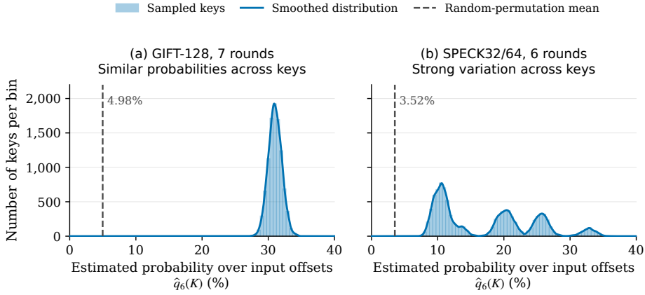
Fig. 18: Key dependence of divisibility by 64 on input-extended structures, using 10,000 keys and 2,048 offsets per key in each panel. Both distributions include offset-sampling variation.
