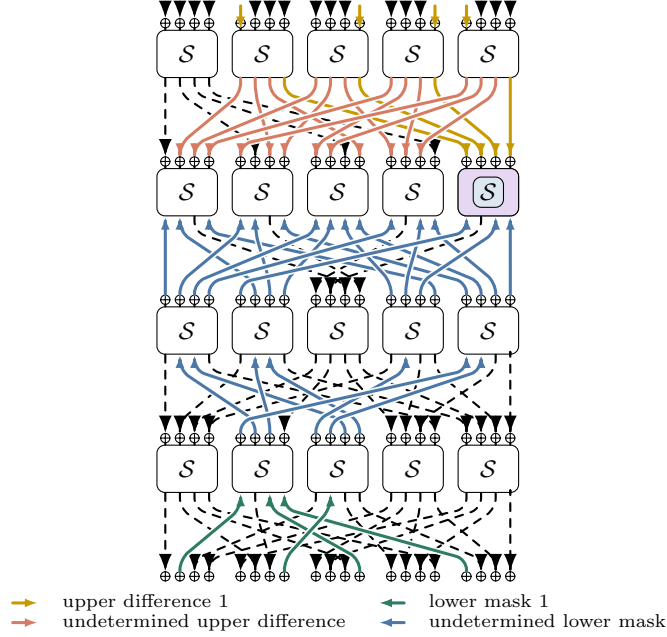
Fig. 7: A larger PRESENT-based ToySPN counterexample: the local DLCT-zero criterion rejects (\delta, \beta) = (08118, 41108) , although the exact sum need not vanish.
