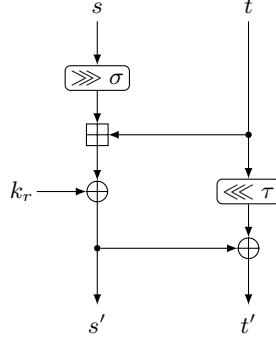
Fig. 9: The SPECK round function.
