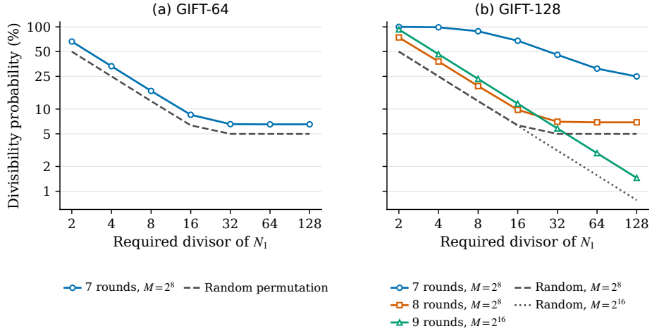
Fig. 15: GIFT-64 and GIFT-128 divisibility probabilities, following the conventions of Figure 14. Round counts include the input-side extension.
