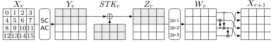
Fig. 13: A round of SKINNY-64 . Cell j contains global bits 60 - 4j, \dots, 63 - 4j .
