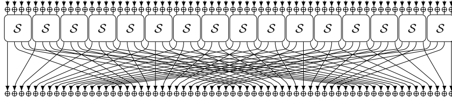
Fig. 10: A round of PRESENT.
