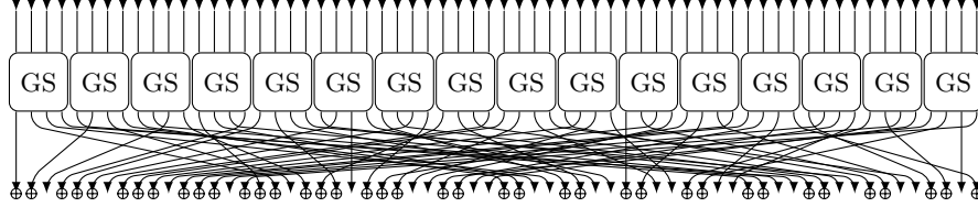
Fig. 12: A round of GIFT-64.
