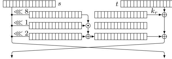
Fig. 8: The SIMON round function, drawn for w = 16 . s is the left word and t the right word.
