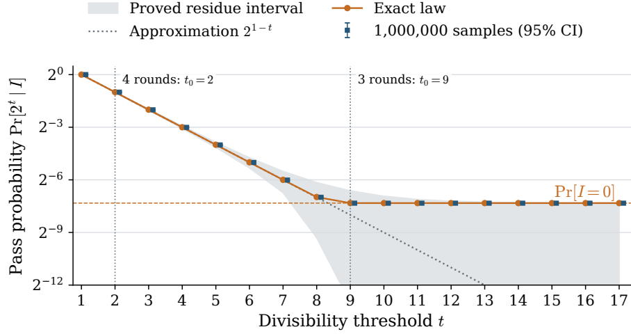
Fig. 5: Shared random-permutation baseline for the 3- and 4-round four-S-box examples: n = 16 and data complexity 2^{15} . Samples are independent draws from the one-coset hypergeometric law. Error bars are pointwise 95% Wilson intervals, not simultaneous confidence bands.
