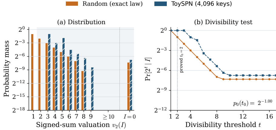
Fig. 4: Signed integral sums for the 4-round, four-S-box ToySPN. The cipher plateau includes the 38 sampled zero sums, which satisfy every divisibility threshold.
