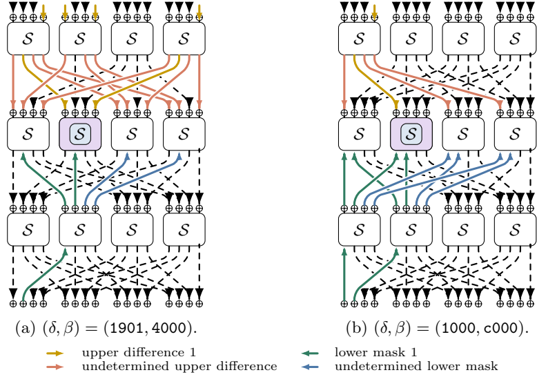
Fig. 6: Local DLCT zeros do not imply fixed-key ZCDL in these 3-round KNOT-S-box ToySPN examples. Local bit patterns are read least-significant bit first. Endpoint masks use the packed convention of Subsection D.1.
